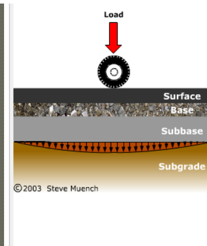
Figure 1. Flexible pavement load distribution.
